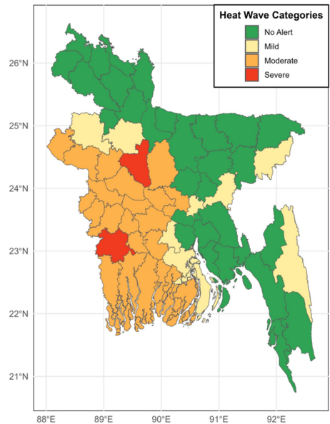
Observed Heat Wave (28 March 2025)
