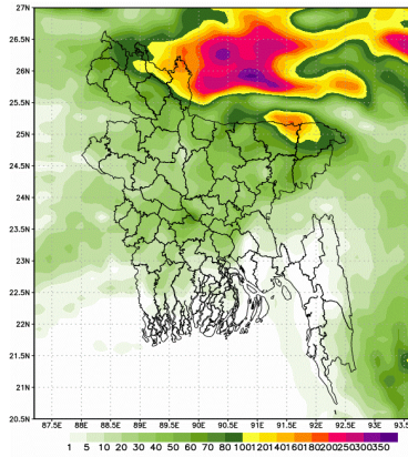
Accumulated Rainfall (mm) Period (12-05-2025 to 17-05-2025)
